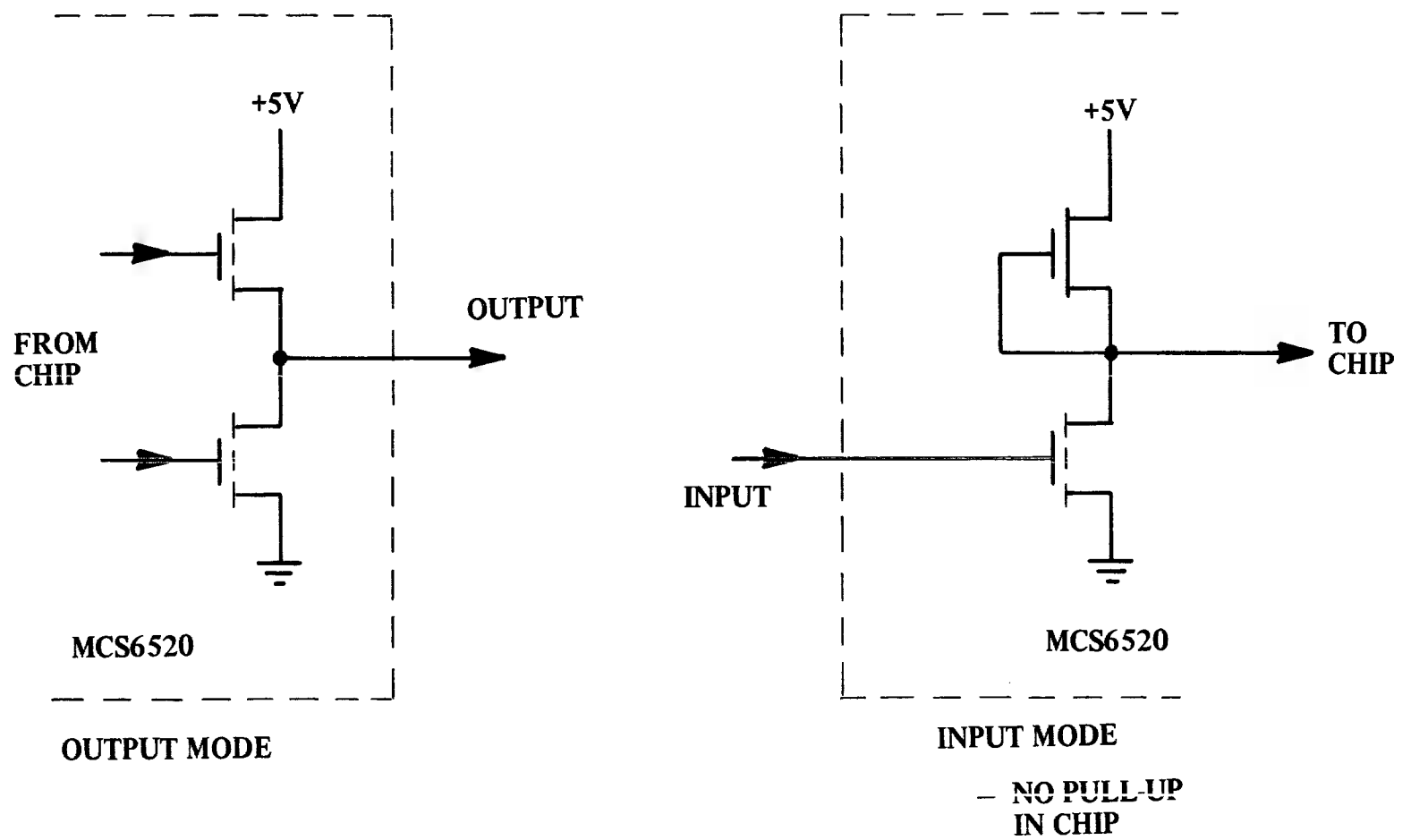
Peripheral I/O Port B Buffer FIGURE 1.28B
